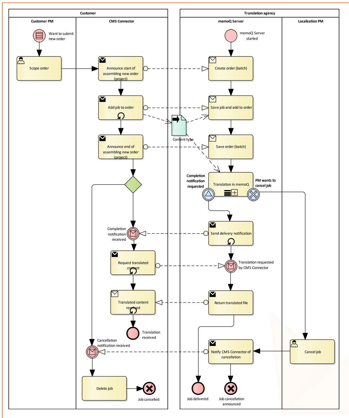
Figure 7. Workflow of translation via memoQ
