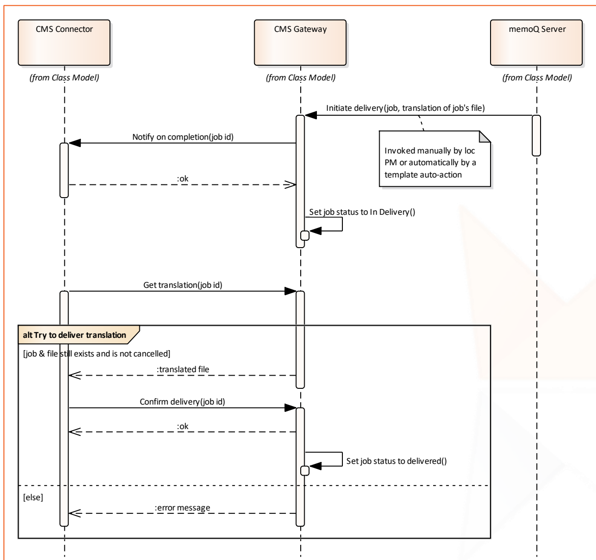
Figure 11. Collaboration protocol of delivering jobs
