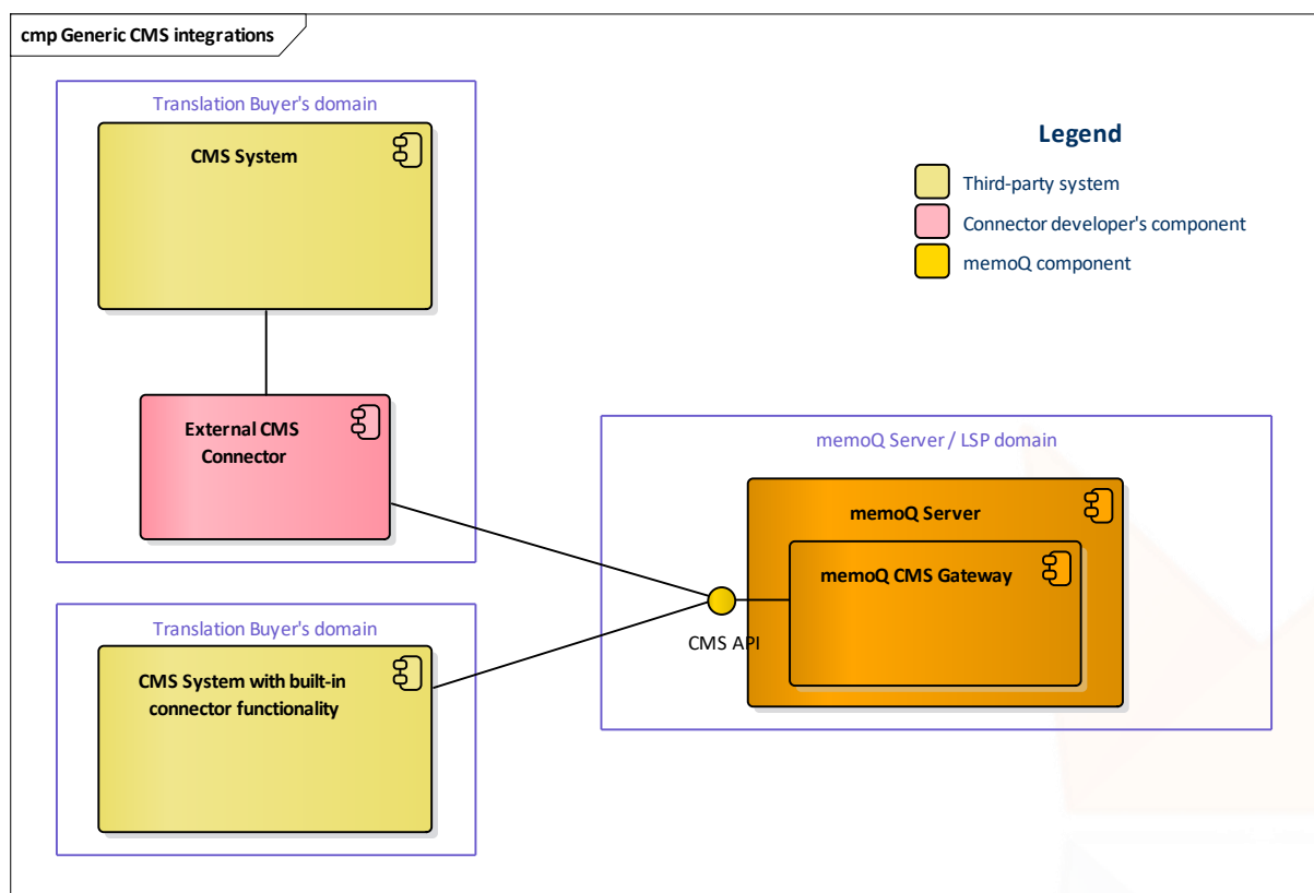
Figure 1. Architecture of CMS integration solutions
