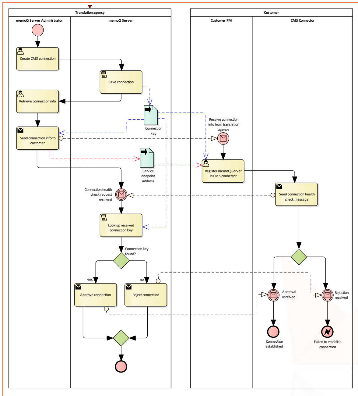
Figure 6. Workflow of setting up a CMS connection
