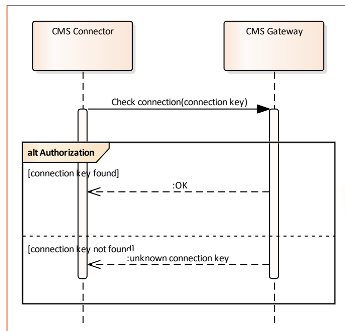
Figure 9. Collaboration protocol of performing connection health check
