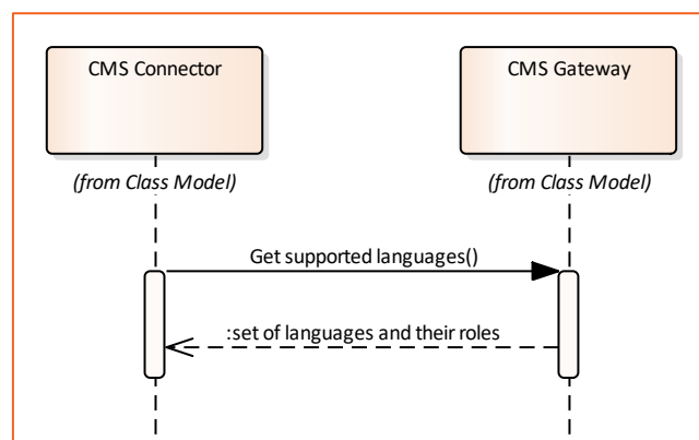
Figure 15. Collaboration protocol of getting list of supported languages
