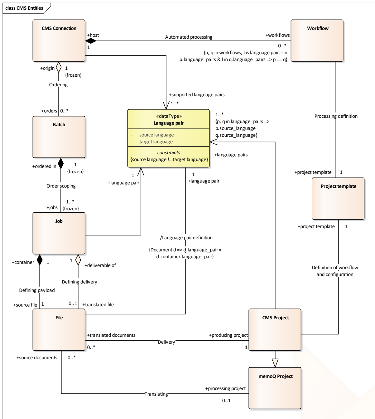
Figure 3. CMS domain model
