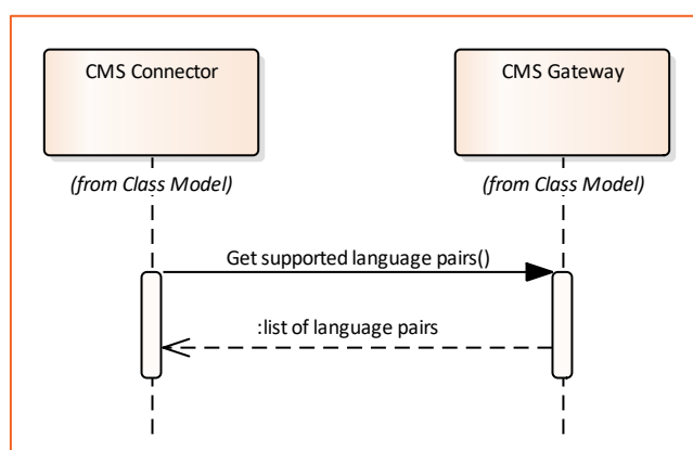
Figure 16. Collaboration protocol of getting the list of language pairs supported by the CMS connection
