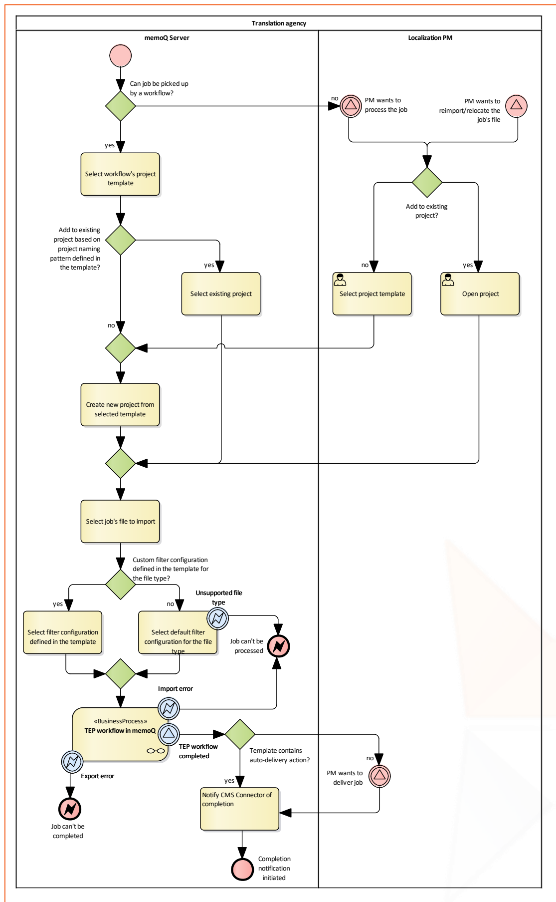
Figure 8. Workflow of translation in memoQ
