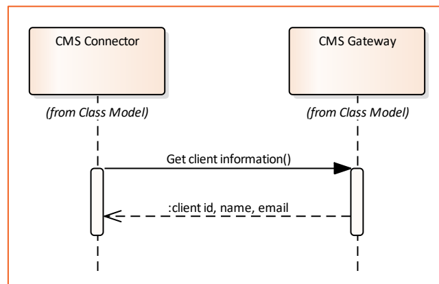
Figure 14. Collaboration protocol of getting client information
