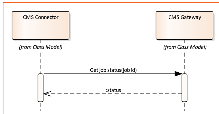
Figure 13. Collaboration protocol of getting CMS job status information
