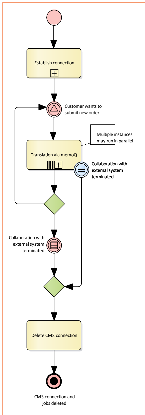
Figure 5. CMS Connection lifecycle workflow
