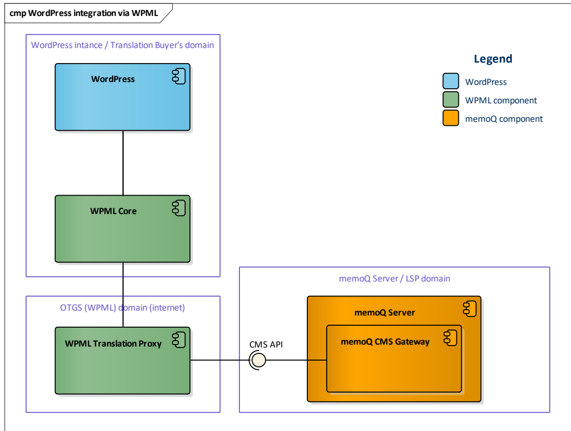
Figure 2. Architectural view of WordPress-memoQ integration via WPML Translation Proxy
