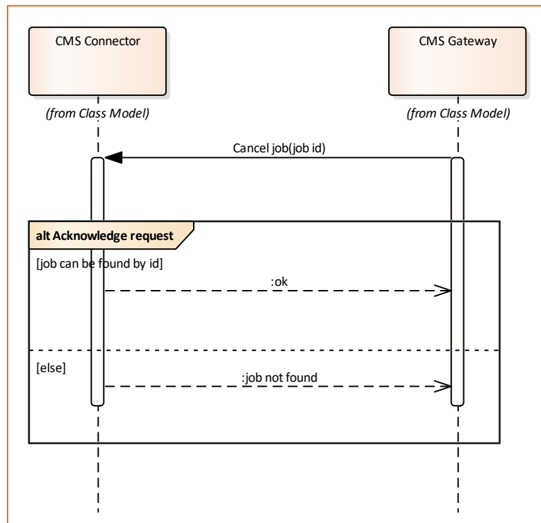
Figure 12. Collaboration protocol of cancelling a job by memoQ Server
