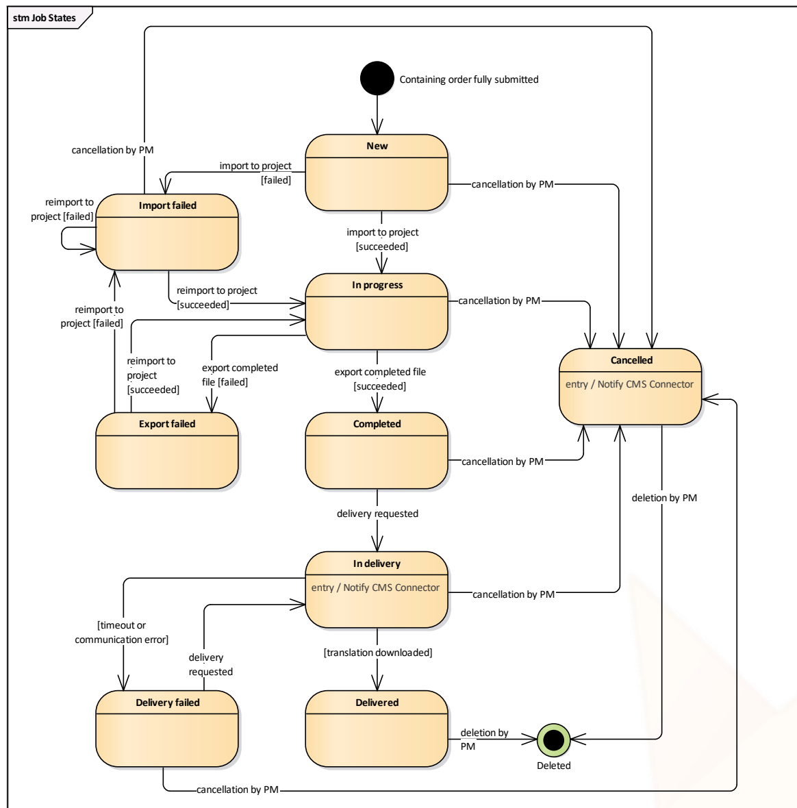
Figure 4. CMS Job states
