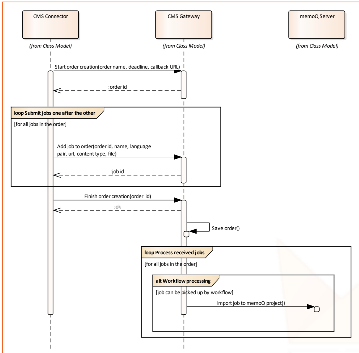
Figure 10. Collaboration protocol of submitting orders
